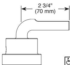
RP72604 Available Extension Kit
