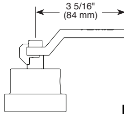
HL6634-▲ Industrial Lever Handle
