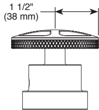
HW6632-▲ Wheel Handle
