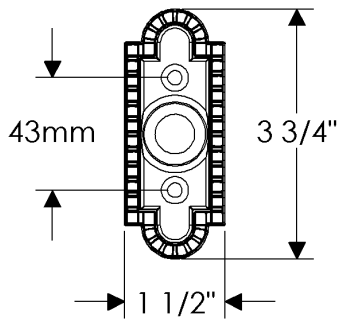
EW30600 Corbel Arched Escutcheon 1 1/2" x 3 3/4"
